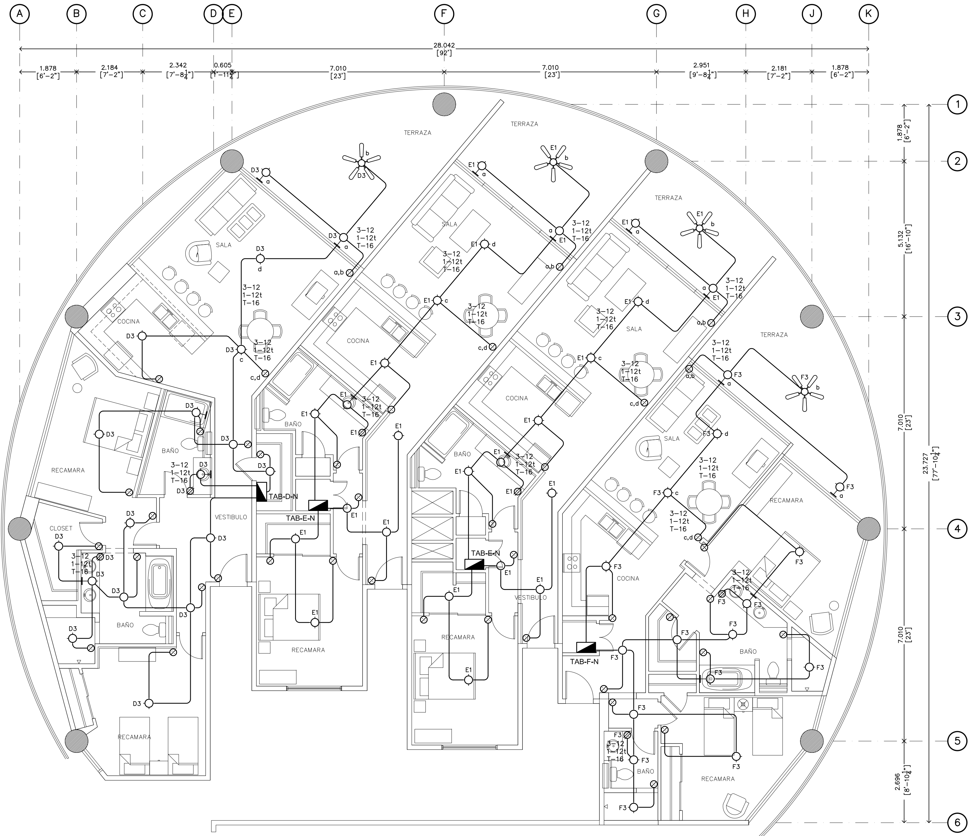
ALUMBRADO KNUCKLE 4 RECAMARAS..... Esc: 1:75
