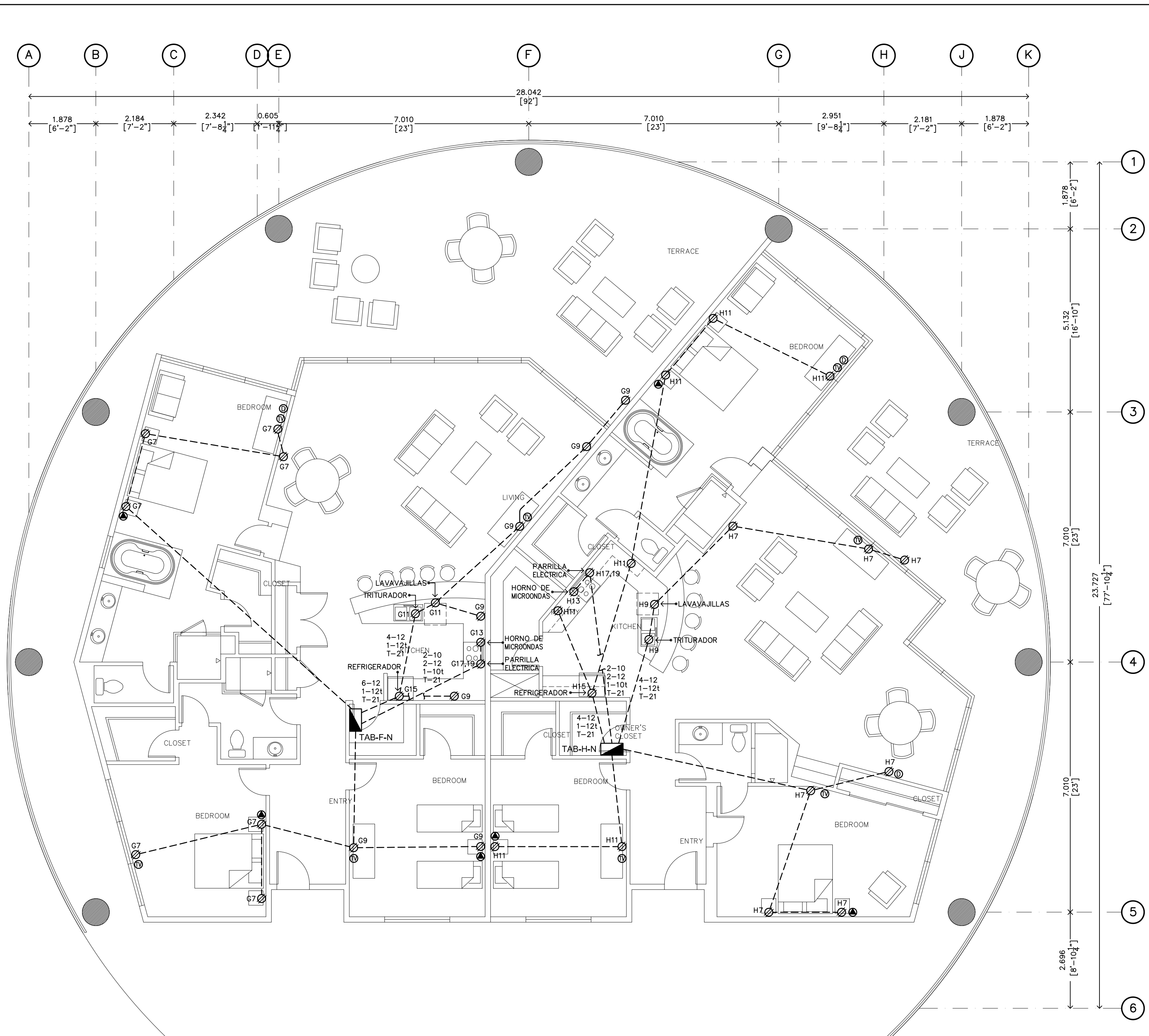
RECEPTACULOS KNUCKLE 2 RECAMARAS..... Esc: 1/75
